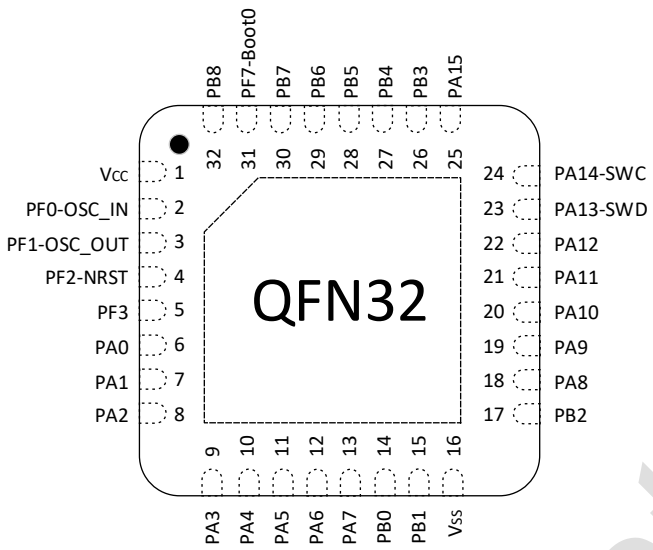
图 3-7 QFN32(4*4) Pinout2 PY32F031K2xU7 (Top view)
