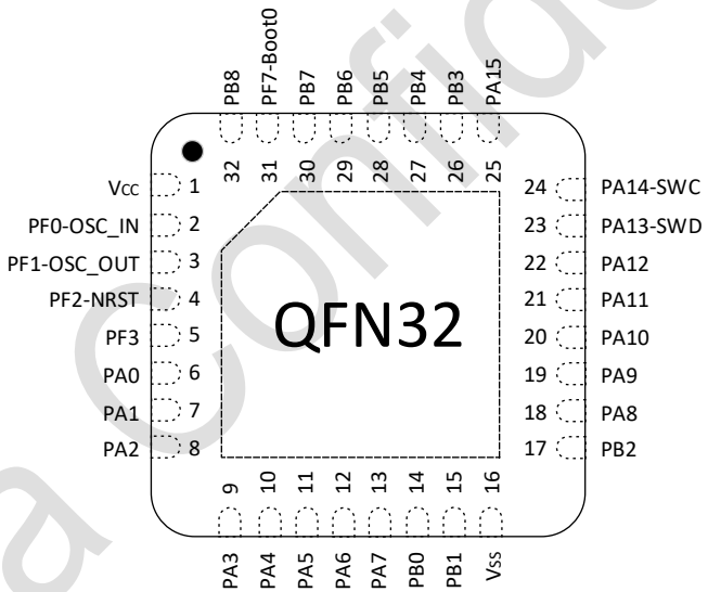
图 3-6 QFN32(5*5) Pinout1 PY32F031K1xU6 (Top view)
