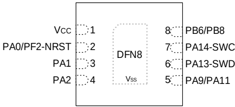
图 3-9 DFN8(2*2) Pinout1 PY32F031L1xD6 (Top view)
