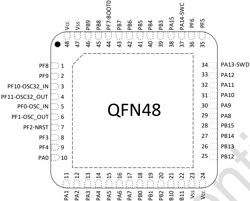
图 3-3 QFN48(5*5) Pinout2 PY32F031C2xU6 (Top view)
