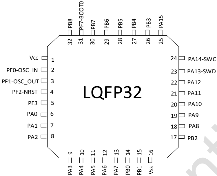
图 3-5 LQFP32 Pinout1 PY32F031K1xT6 (Top view)
