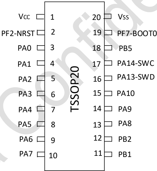
图 3-8 TSSOP20 Pinout1 PY32F031F1xP6 (Top view)
